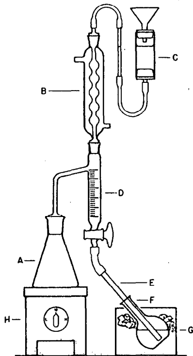
Azeotropic distillation apparatus
